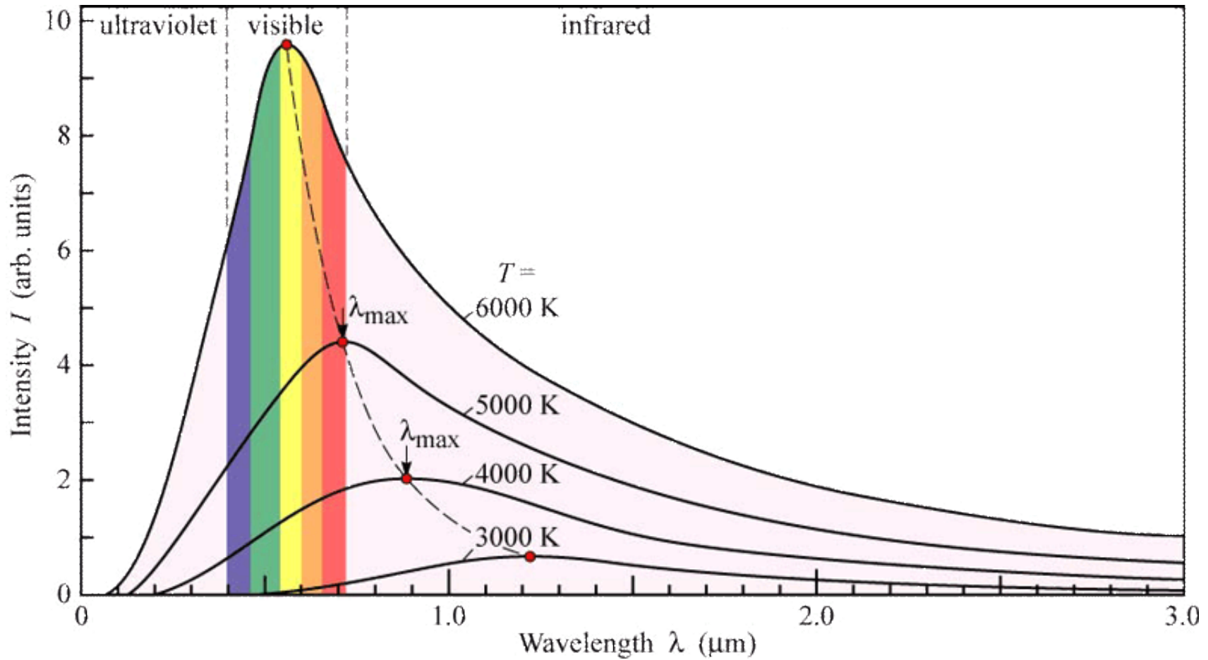
Figure 2: Spectra of black-body radiation at various temperatures, according to Wien's displacement law [2].
